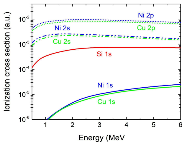
Figure 1: Present CDWEIS results for Si, Ni, and Cu.
