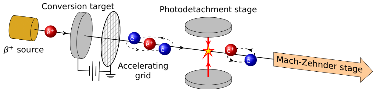
Figure 1: Scheme of the QUPLAS stages to produce the Ps beam as input for the Mach-Zehnder interferometer
