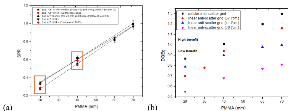
Figure 1 (a) Scatter-to-primary ratio (SPR) without anti-scatter grid as a function of PMMA thickness for a direct-conversion detector (aSe) and an indirect-conversion detector (CsI) (black symbols). The results are compared with simulation data reported [2] (red symbols). (b) Grid detective quantum efficiency (DQE g ) as a function of PMMA thickness for different anti-scatter grid designs.
