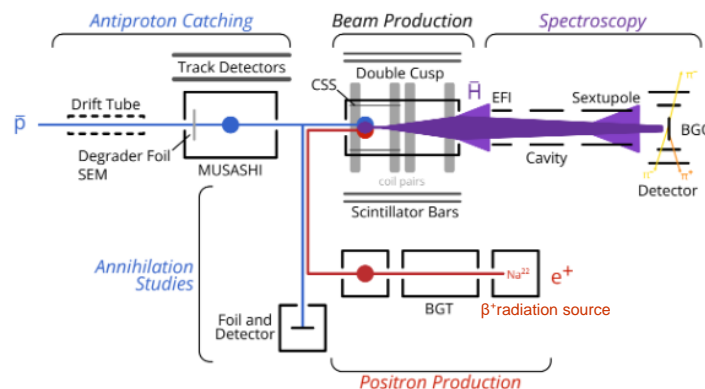
Figure 1. Overview of the ASACUSA hyperfine spectroscopy beamline.
